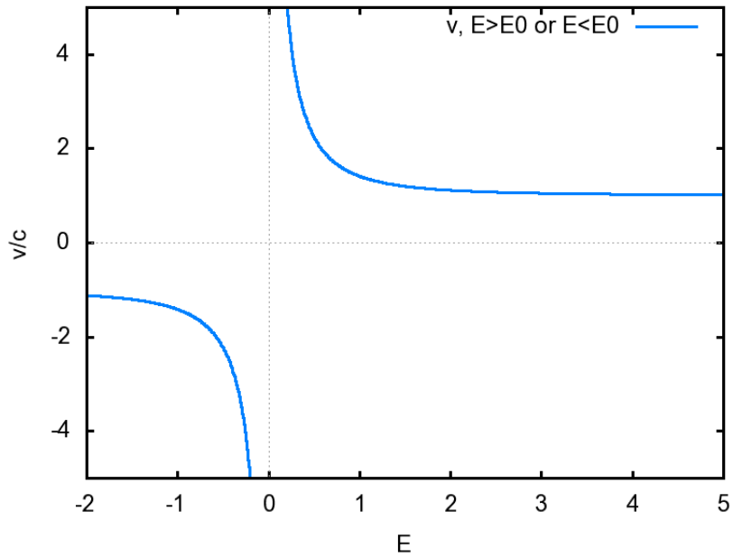
Figure 2: Energy dependence of v/c for imaginary mass, m = c = E_0 = 1 .
