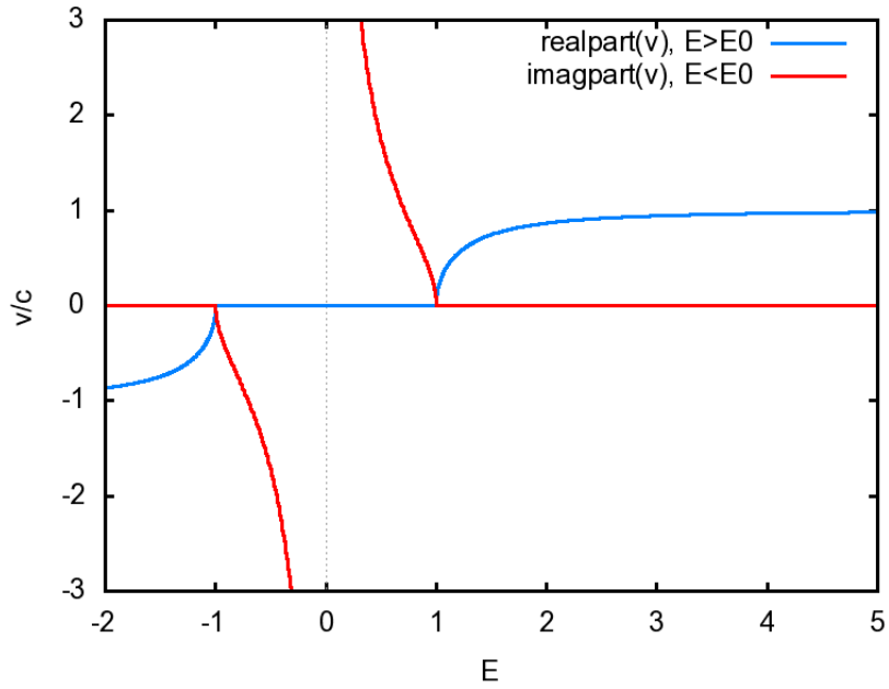
Figure 1: Energy dependence of v/c , real and imaginary parts for m = c = E_0 = 1 .
