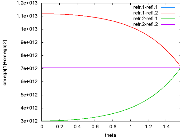
Figure 3: Summed frequencies \omega_1 + \omega_2 from Figs. 1 and 2.
