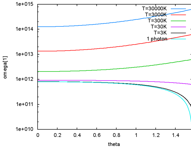
Figure 4: Temperature dependence of refracted frequency \omega_1 .
