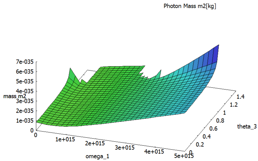
Figure 10: Calculated photon mass in dependence of \omega_1 and \theta_3 , second solution.
