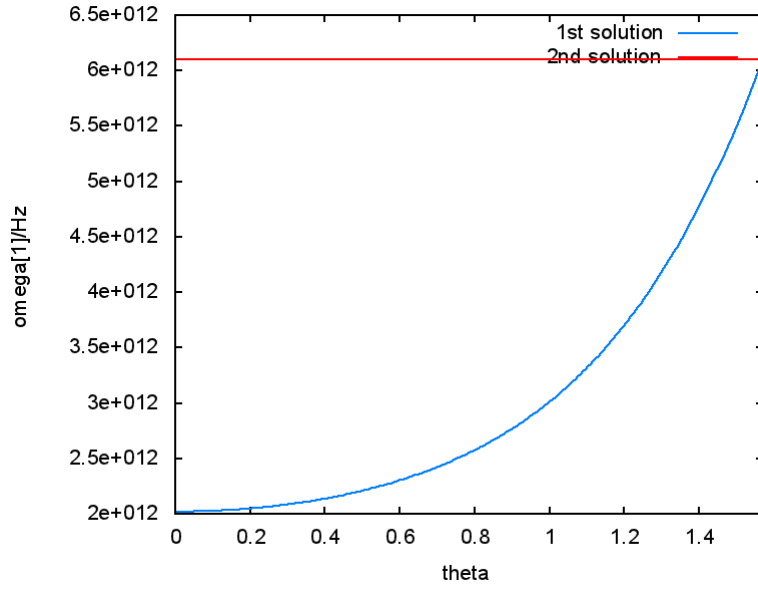
Figure 1: The two solutions for \omega_1 . Parameters see text.
