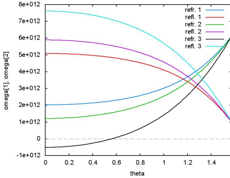
Figure 5: Refracted and reflected frequencies \omega_1 and \omega_2 for three parameter choices of a complex refractive index (Eqs.(75-77)).
