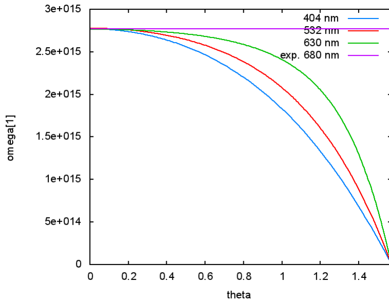
Figure 8: Refracted frequencies \omega_1 for olive oil with parameters taken from Table 2.
