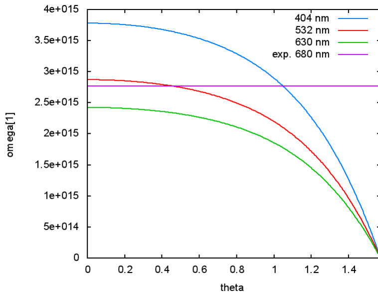
Figure 6: Refracted frequencies \omega_1 for olive oil, n_1 = 1.4665 .
