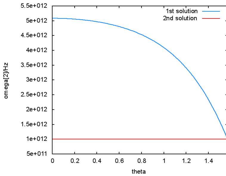
Figure 2: The two solutions for \omega_2 . Parameters see text.
