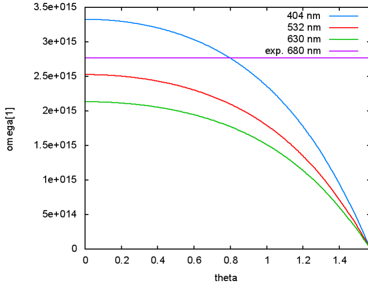
Figure 7: Refracted frequencies \omega_1 for olive oil, n_1 = 1.959 .
